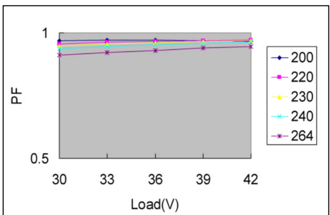
PF curve
