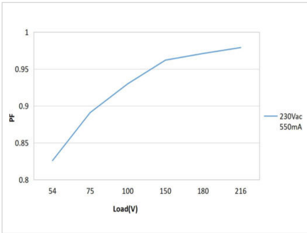
PF Curve 5
