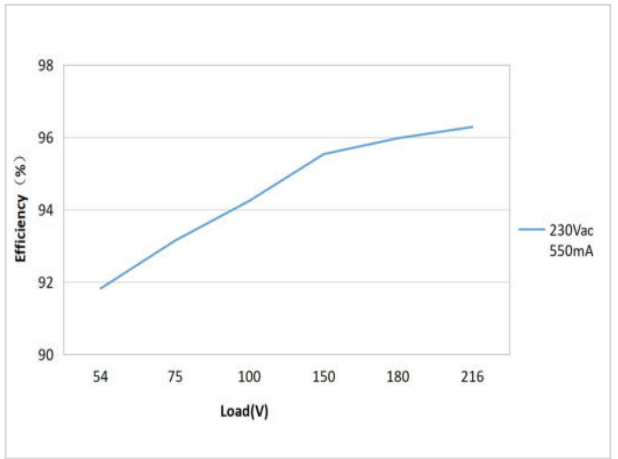
Efficiency Curve 5
