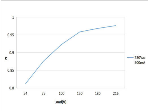
PF Curve 7
