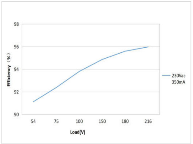
Efficiency Curve 9
